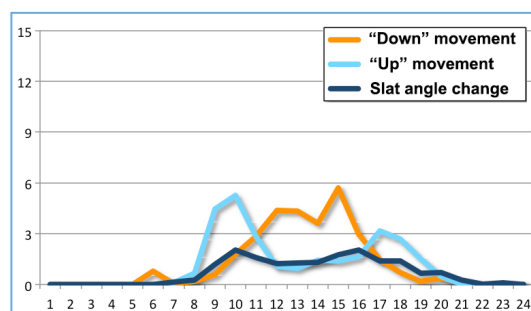
Figure 5: SOUTH façade: Daily distribution of blind movement
