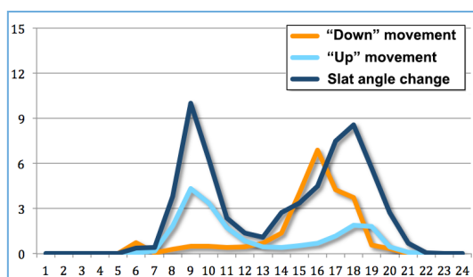
Figure 7: WEST façade: Daily distribution of blind movement
