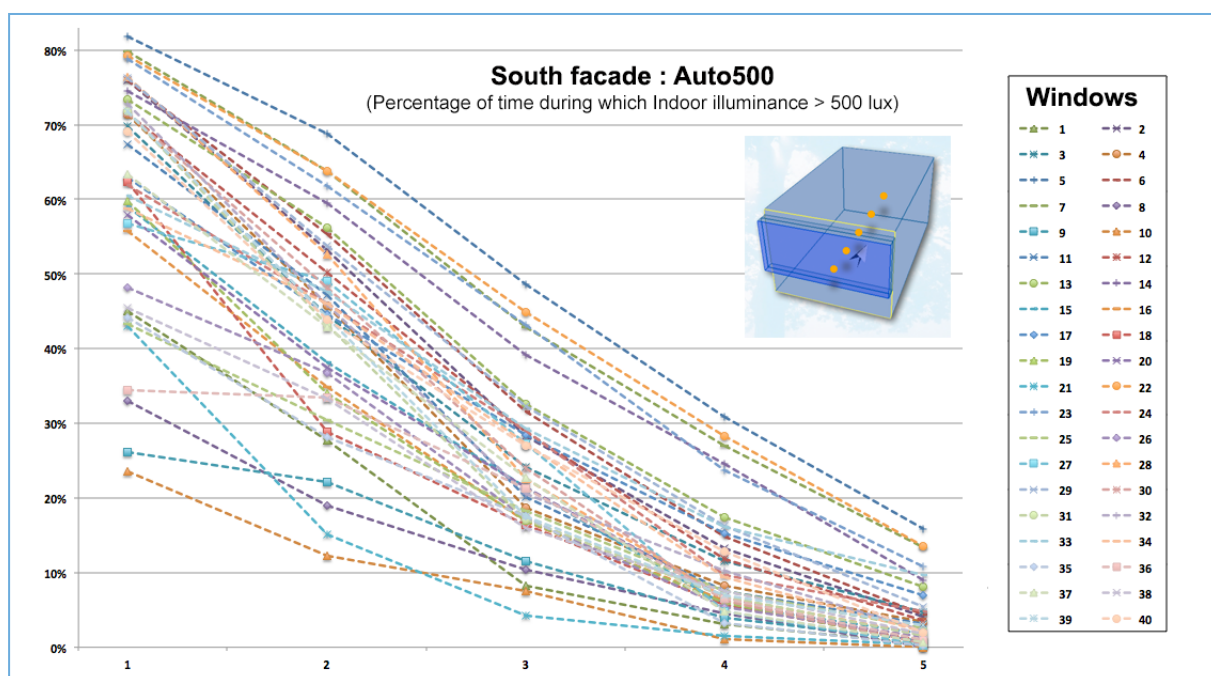
Figure 9: Percentage of the time (7 AM- 6 PM), during which daylight contribution \geq 500 lux on the five reference points, for each of the 40 south oriented rooms. Each line corresponds to a room. Point 1 (left), is located close to the window and point 5 (right) is at the back of the room.
